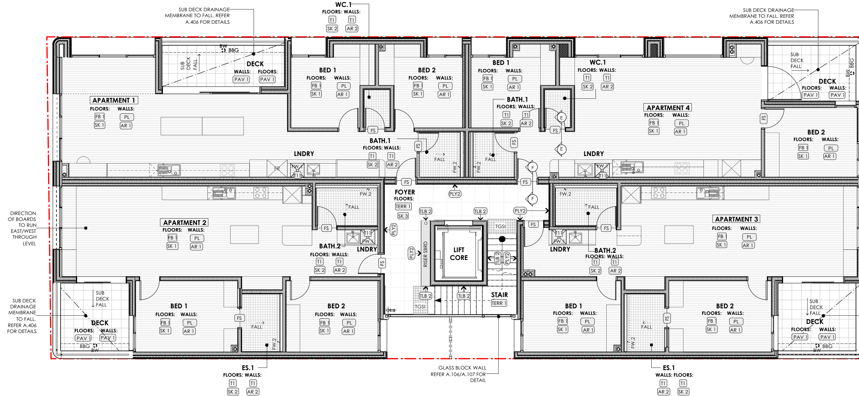
2 FINISHES PLAN - LEVEL 01 SCALE: 1:100
