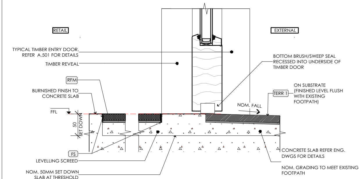
B RETAIL/ENTRY THRESHOLD Scale: 1:5
