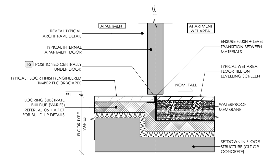
E TYPICAL APARTMENT WET AREA THRESHOLD Scale: 1:5
