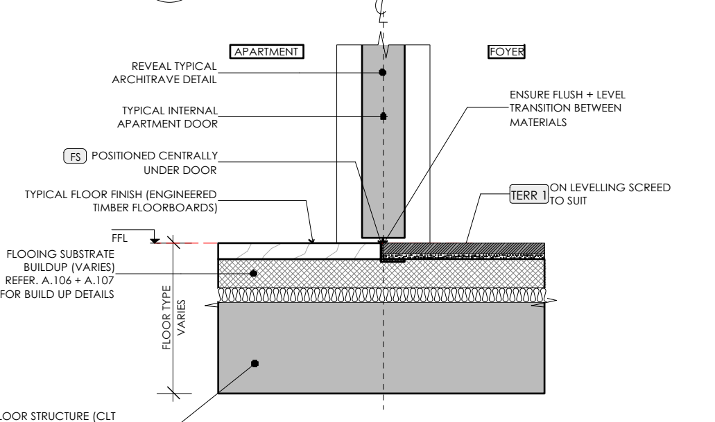
F TYPICAL APARTMENT/FOYER THRESHOLD Scale: 1:5
