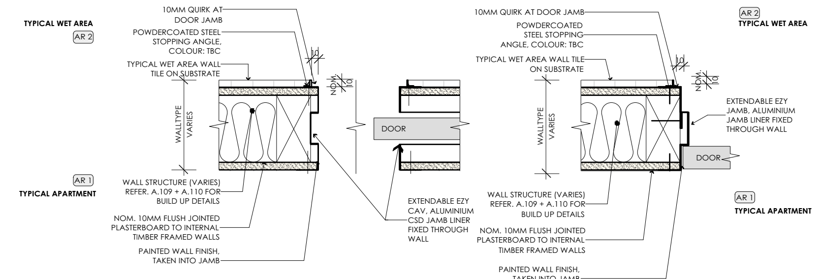
I TYPICAL ARCHITRAVE DETAILS Scale: 1:5
