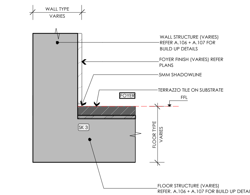
H SKIRTING TYPE 3 Scale: 1:5
