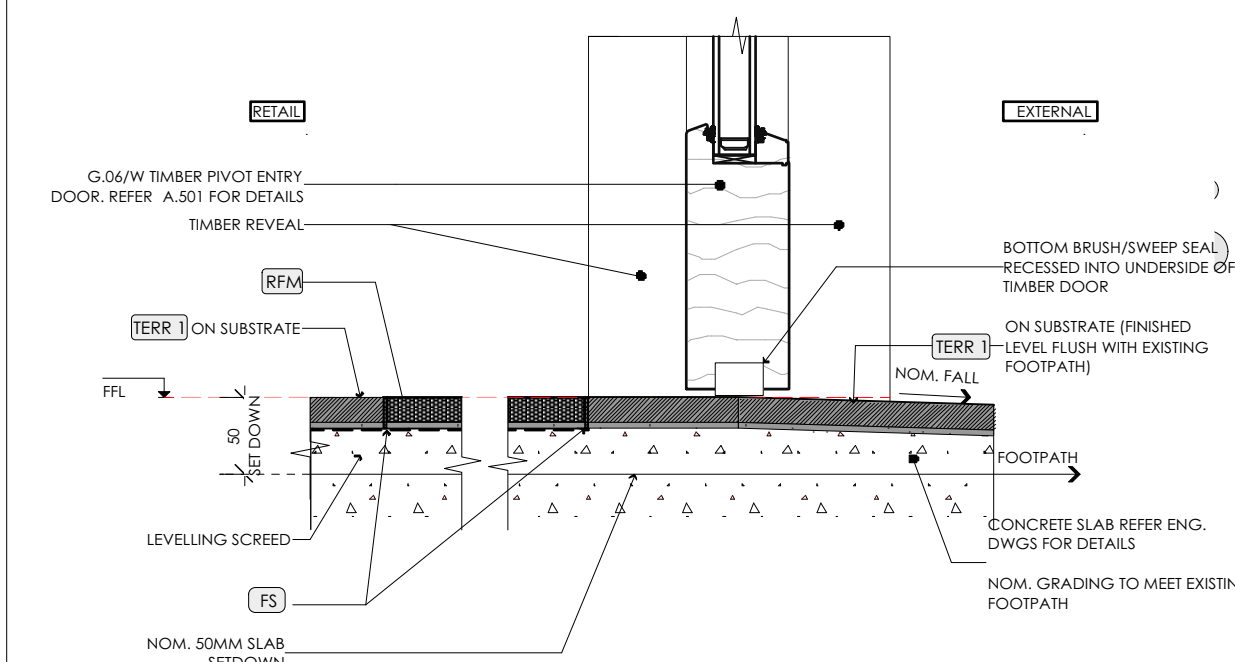
C FOYER/ENTRY THRESHOLD Scale: 1:5
