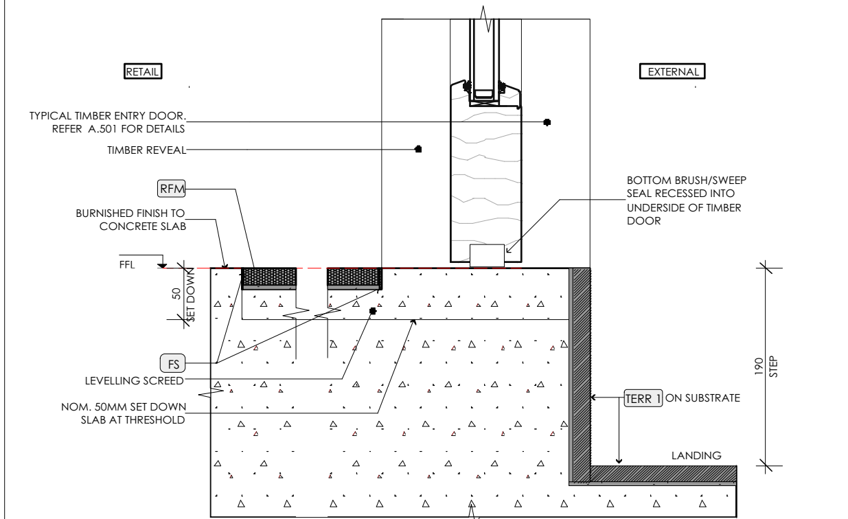
A RETAIL/ENTRY THRESHOLD Scale: 1:5
