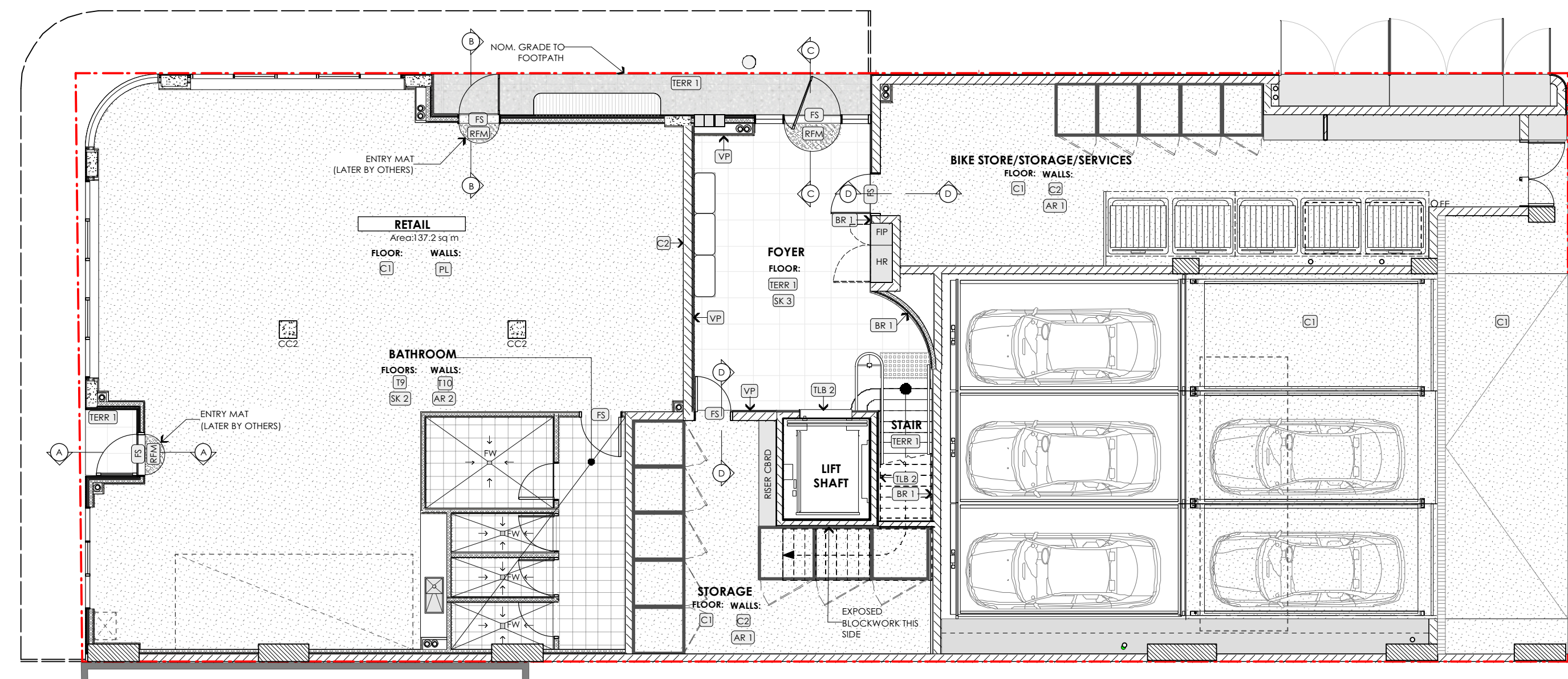
1 FINISHES PLAN - LEVEL GR SCALE: 1:100
