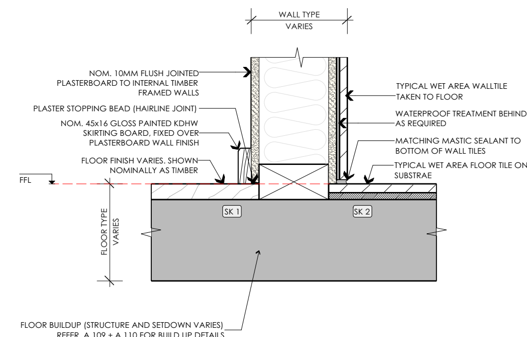
G SKIRTING TYPE 1 + 2 Scale: 1:5
